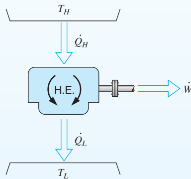
FIGURE 5.25 A heat engine operating between two constant-temperature energy reservoirs for Example 5.4.
