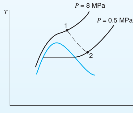
FIGURE 12.10 Sketch for Example 12.6.
