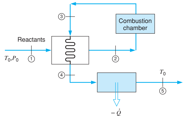
FIGURE P13.97
