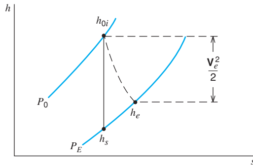
FIGURE 15.19 An h - s diagram showing the effects of irreversibility in a nozzle.
