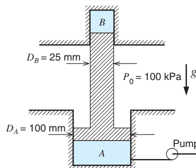
FIGURE P1.100
