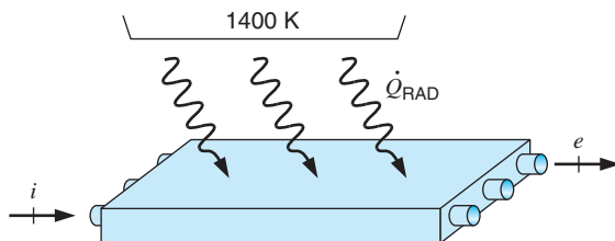
FIGURE P11.54
