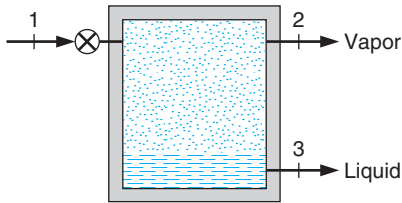
FIGURE P8.68
