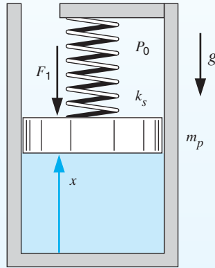
FIGURE 3.10 Sketch of the physical system for Example 3.4.
