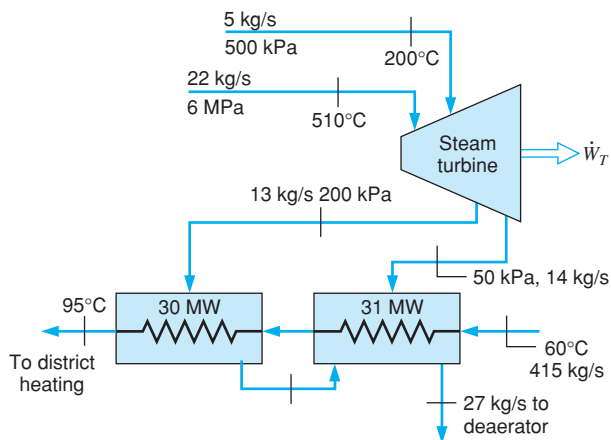
FIGURE P9.80
