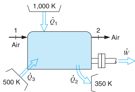
FIGURE P7.35
