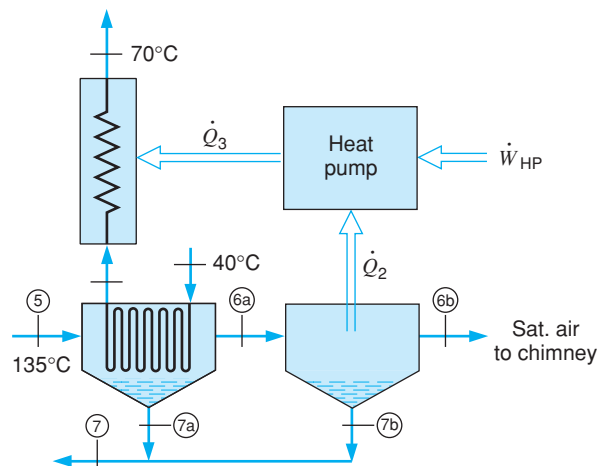
FIGURE P11.194
