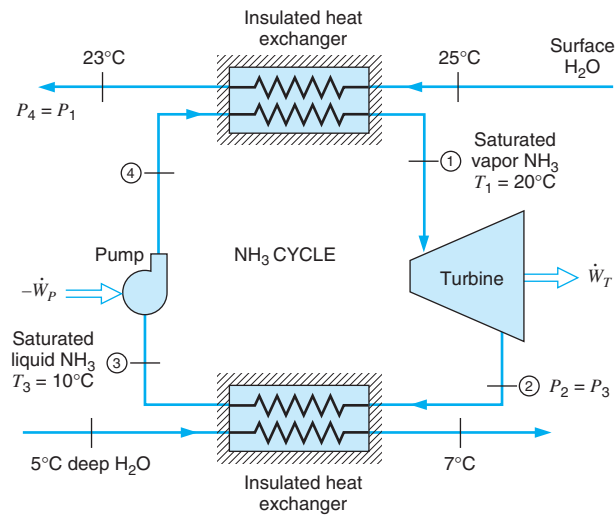
FIGURE P9.31
