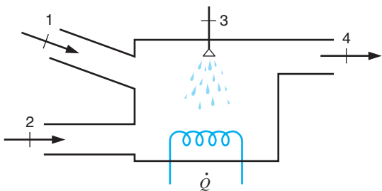
FIGURE P11.142
