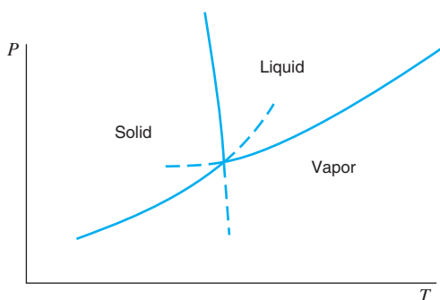
FIGURE 14.5 Metastable states for solid–liquid–vapor equilibrium.
