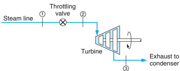
FIGURE P7.39
