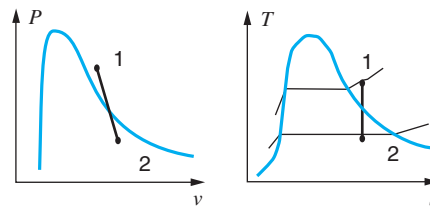
FIGURE P6.8
