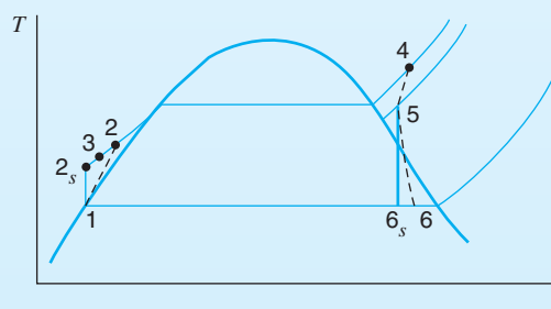
FIGURE 9.18 T - s diagram for Example 9.5.
