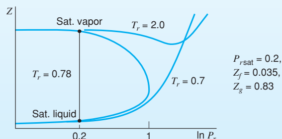
FIGURE 2.21 Diagram for Example 2.11.
