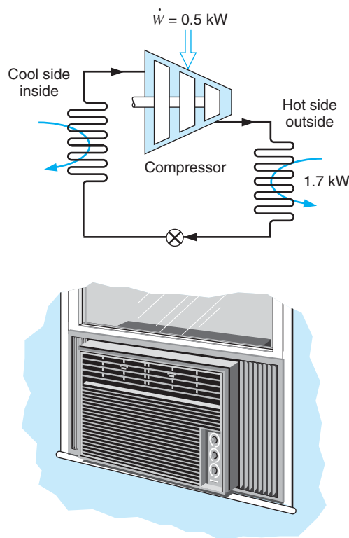
FIGURE P5.23
