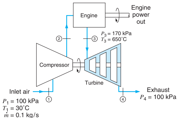
FIGURE P7.41
