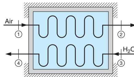
FIGURE P7.105
