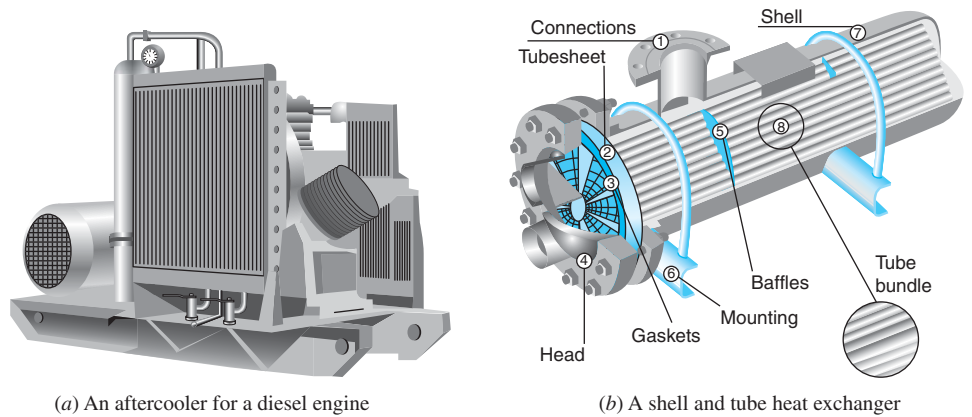
FIGURE 4.18 Heat exchangers.
