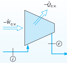
FIGURE 8.7 Illustration for Example 8.2.
