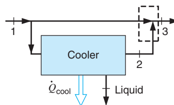
FIGURE P11.95
