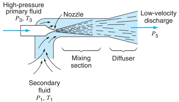
FIGURE P7.172
