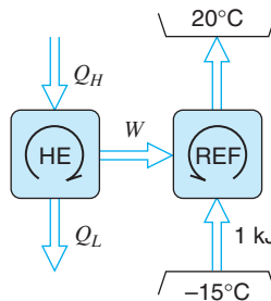
FIGURE P6.38
