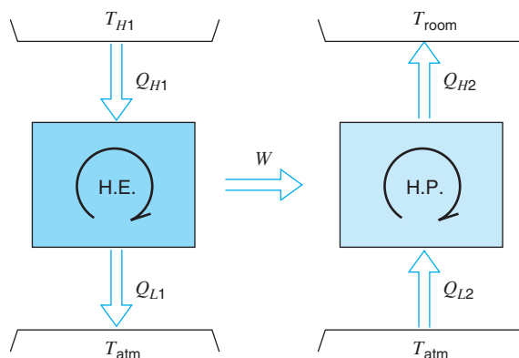
FIGURE P5.115
