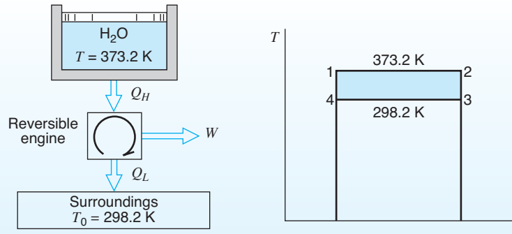
FIGURE 6.20 Reversible heat transfer with the surroundings.
