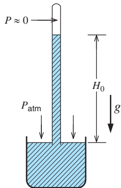
FIGURE 1.14
