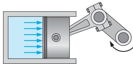
FIGURE P6.111
