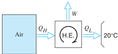
FIGURE P6.99
