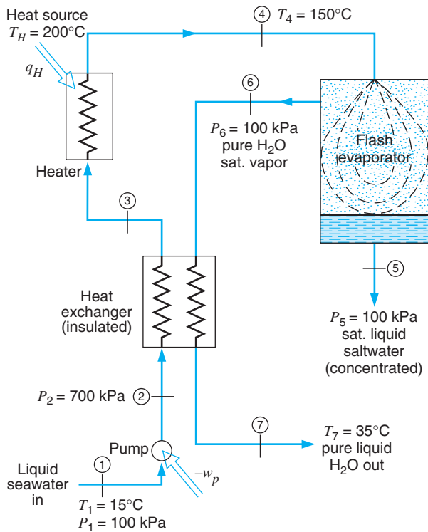
FIGURE P7.170
