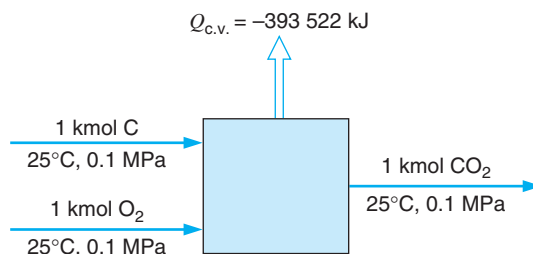
FIGURE 13.3 Example of the combustion process.
