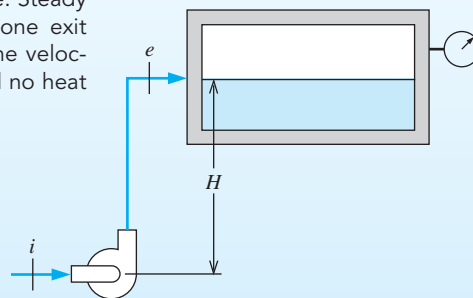
FIGURE 4.10 Sketch for Example 4.6.
