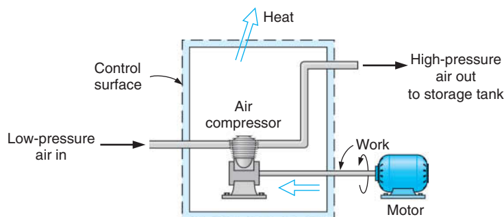
FIGURE 1.5 Example of a control volume.
