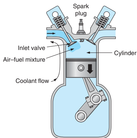
FIGURE P10.73
