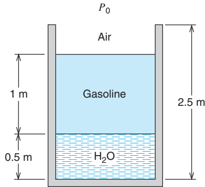
FIGURE P1.55
