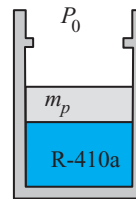
FIGURE P3.237
