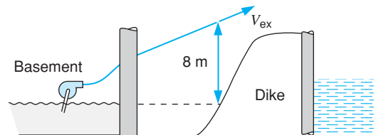
FIGURE P8.34
