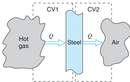
FIGURE P6.115
