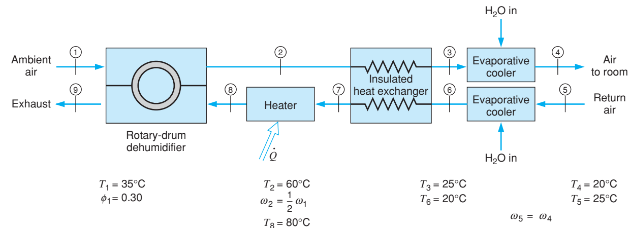
FIGURE P11.144
