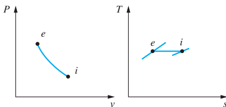
FIGURE P7.4
