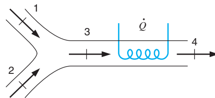
FIGURE P11.114
