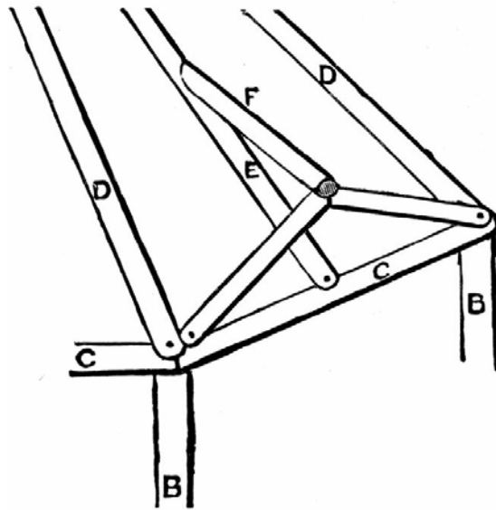
Fig. 176.—Timbers over Entrance of Octagonal Summer-house.
