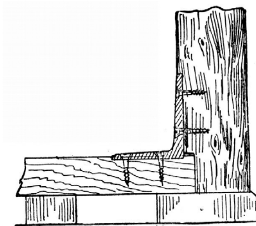
Fig. 166.—Fixing Sleeper to Posts.
