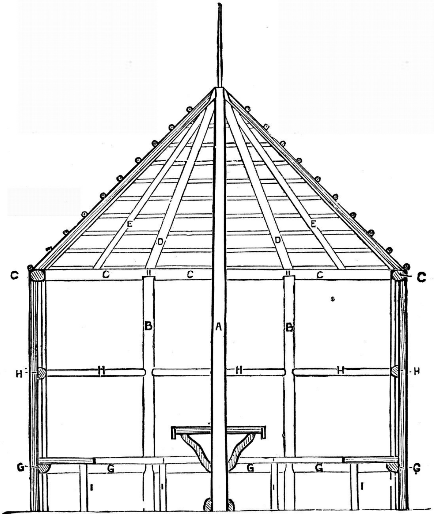
Fig. 174. —Section of Octagonal Summer-house at YZ ( Fig. 173 ), showing Framework.
