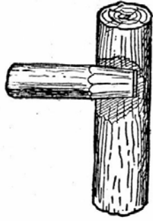
Fig. 126.—Detail of Middle Rail and Post of Foot-bridge.
