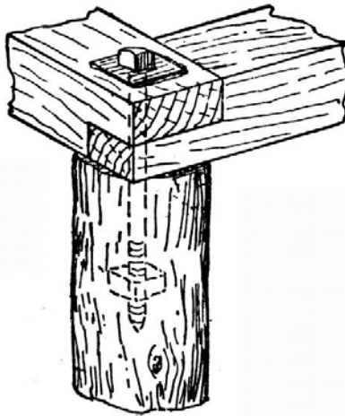
Fig. 165.—Connecting Plates to Corner Post.
