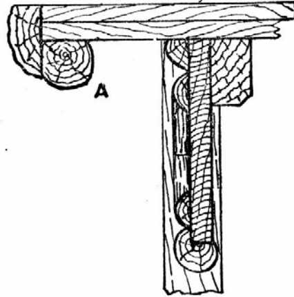
Fig. 100.—Section of Gable for Cottage Porch.
