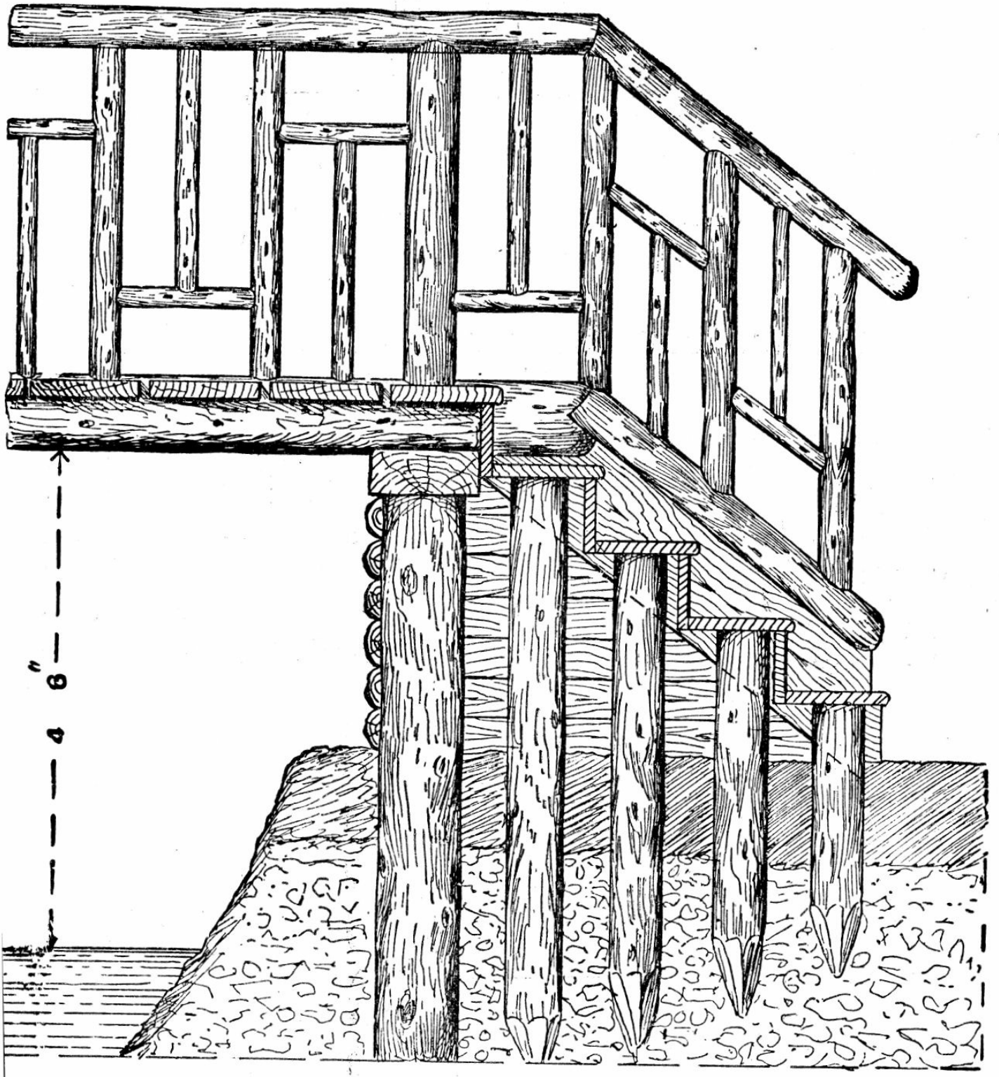
Fig. 130.—Elevated Foot-bridge.
