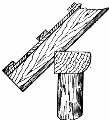
Fig. 98.—Enlarged Detail of Cottage Porch at Eaves.
