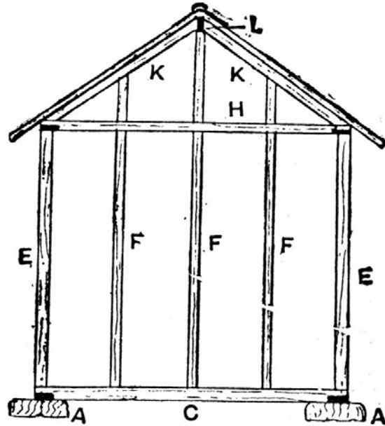
Fig. 144.—Back Framework for Garden Snuggery.
