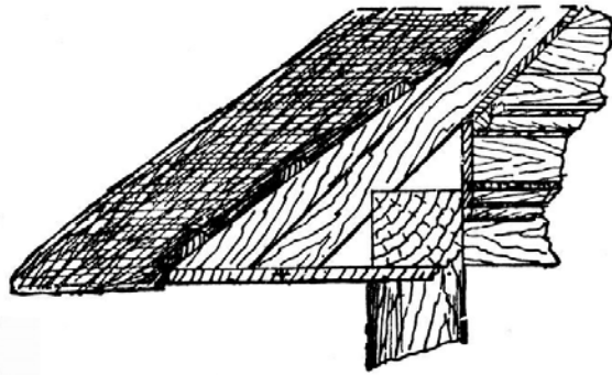
Fig. 169.—Detail of Garden Shelter at Front Eaves.
