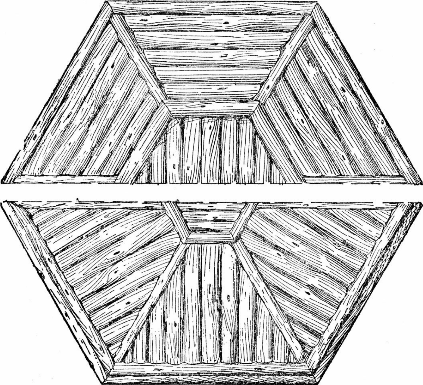
Fig. 45.—Half Plans of Top of Hexagonal Table.
