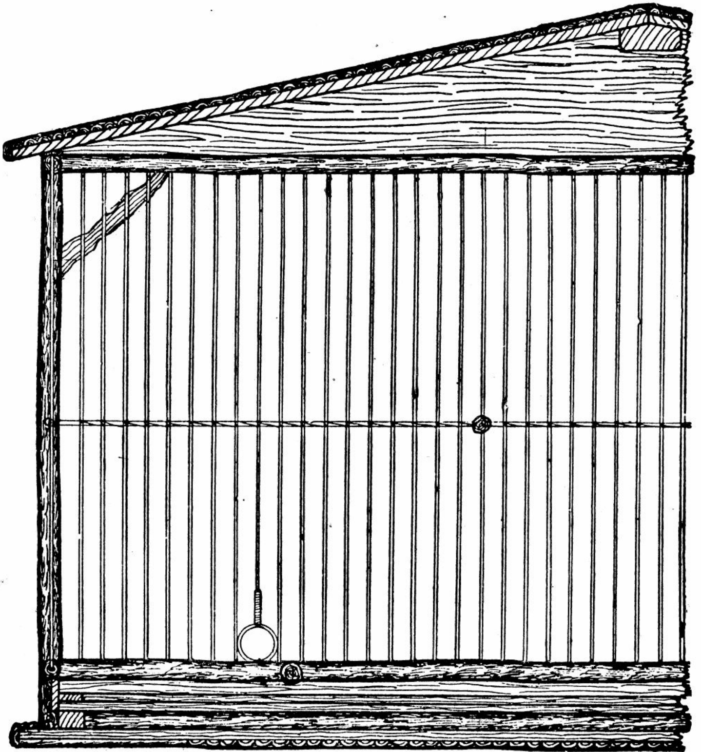
Fig. 119.—Part Longitudinal Section of Aviary.
