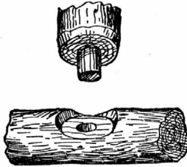
Fig. 155.—Alternative Method of Joining Rails to Posts.
