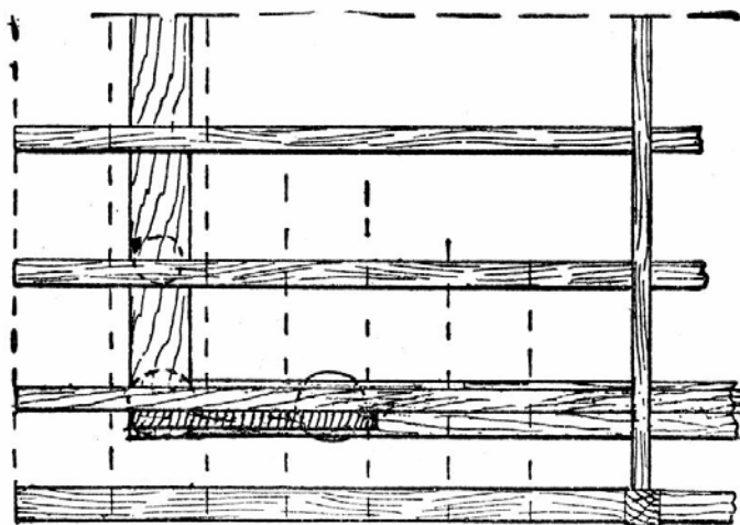
Fig. 99.—Part Plan of Roof for Cottage Porch.
