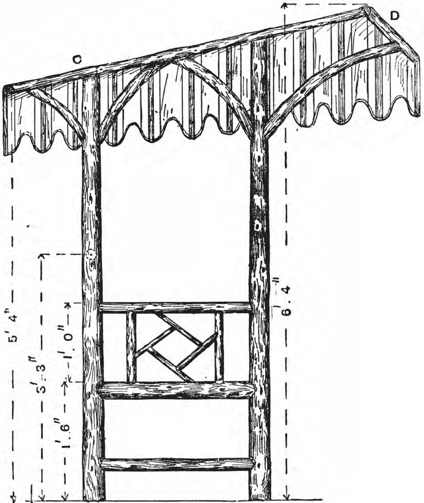
Fig. 151.—Side Elevation of Garden Retreat.
