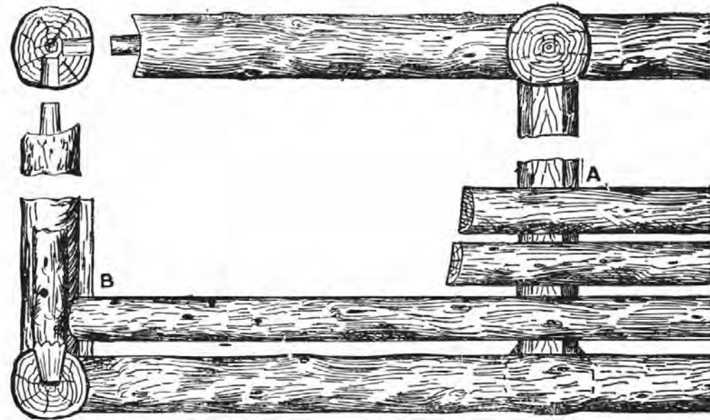
Fig. 152.—Detail of Seat of Garden Retreat.
