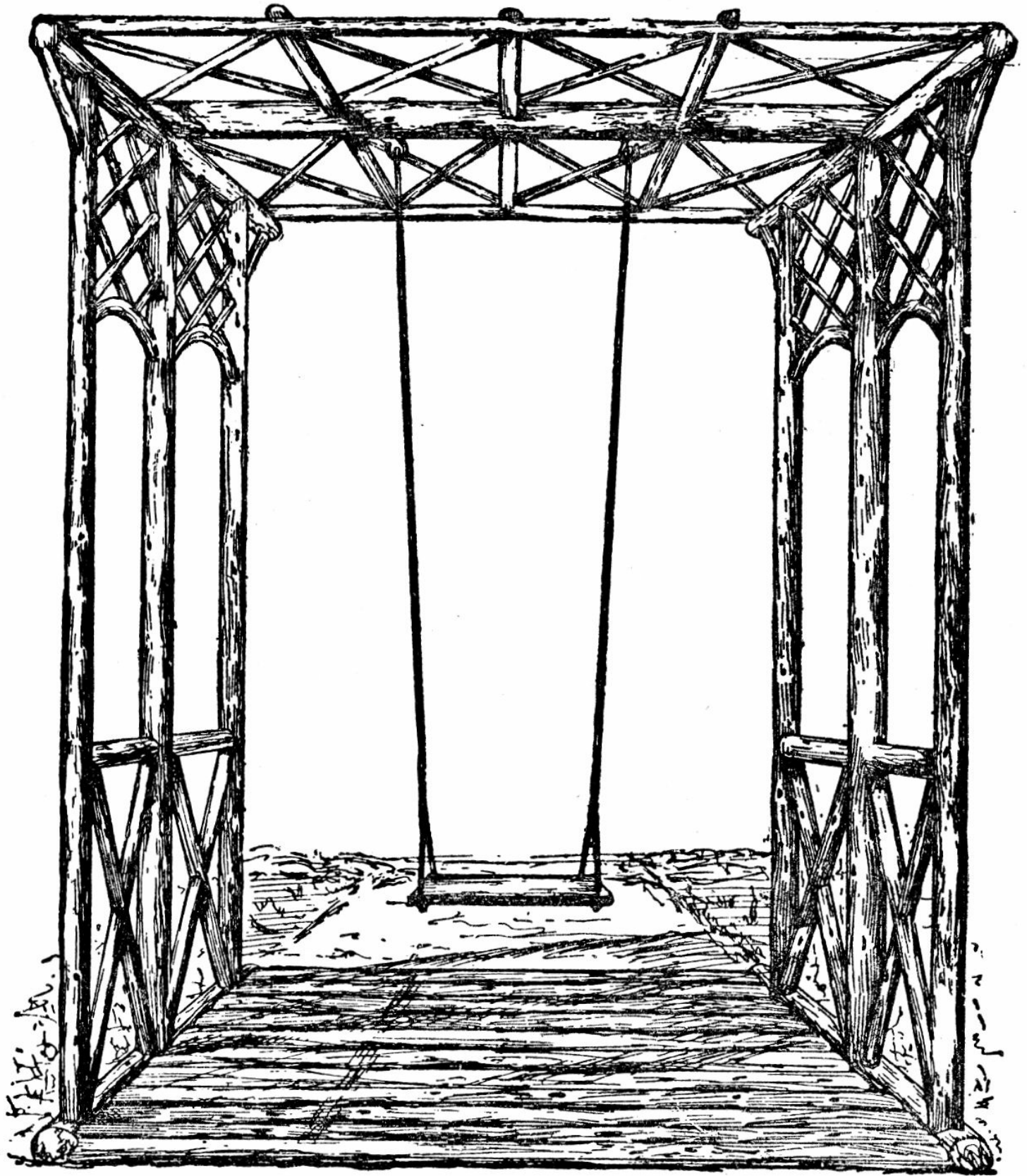
Fig. 101.—General View of Rustic Canopy for Swing.
