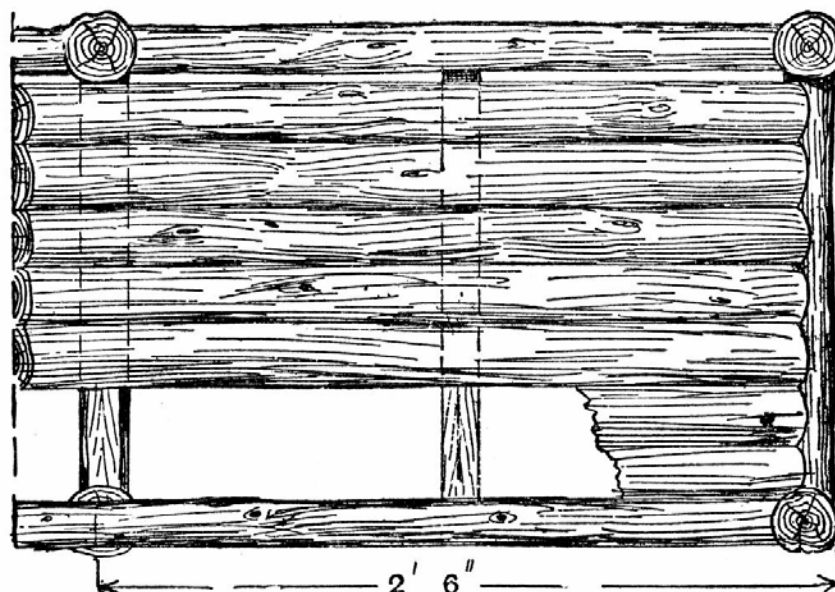
Fig. 57.—Part Plan of Seat.
