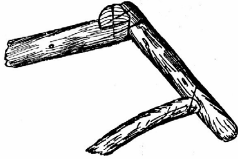
Fig 154.—Detail of Front Joints (See C, Fig. 151).
