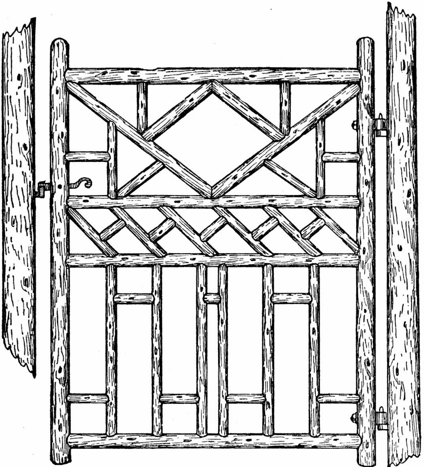
Fig. 86.—Alternative Design for Gate.
