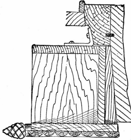
Fig. 16.—Gross Section of Window Box in Position.
