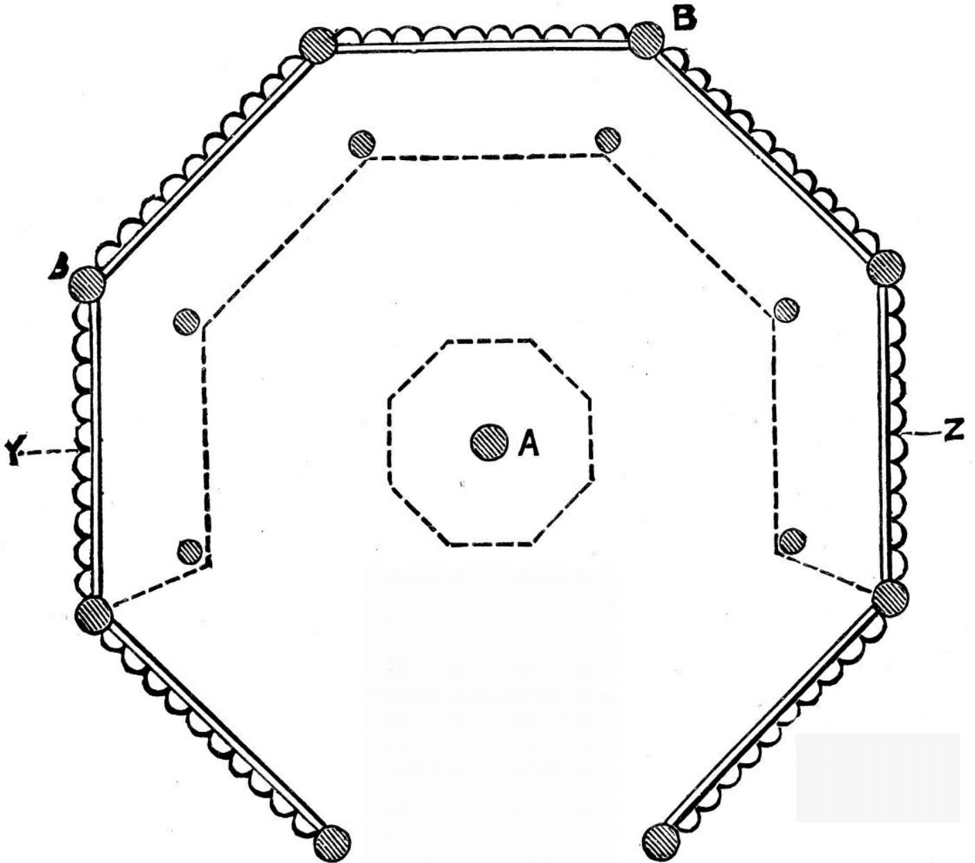
Fig. 173. —Ground Plan of Octagonal Summer house.
