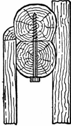
Fig. 123.—Enlarged Section of Girders for Foot-bridge.
