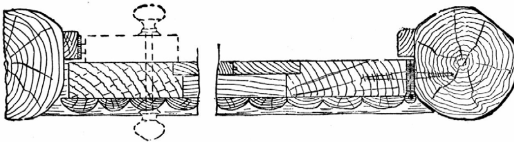
Fig. 191.—Horizontal Section through Door Posts.
