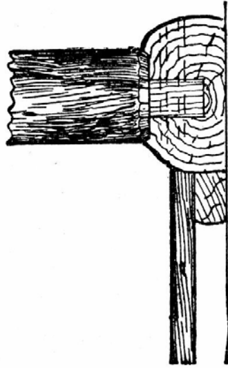
Fig. 103.—Fixing Middle Post of Canopy to Sill.
