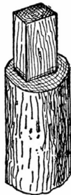
Fig. 125.—Parts of Joint of Post and Girder.
